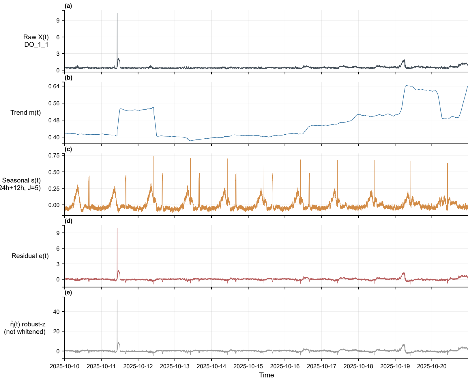
Multi-scale decomposition — DO_1_1 (aerobic, min) [2025-10-10~2025-10-20]
